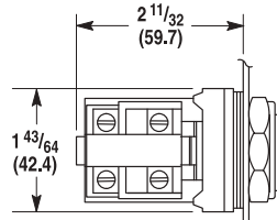
Snap Action Contact Block (For Push Button Only)
