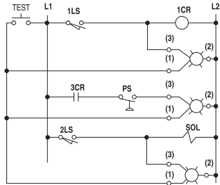
Dual Input Pilot Light Typical Application Wiring Diagram
