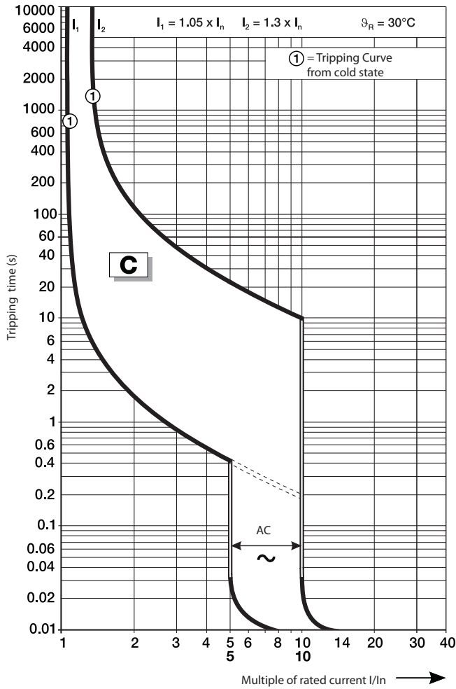
C Curve
