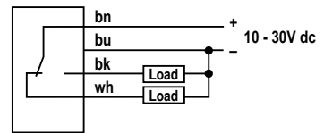
PNP (Sourcing) Outputs Standard Hookup
