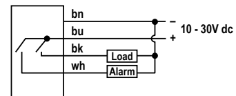
PNP (Sourcing) Outputs Alarm Hookup
