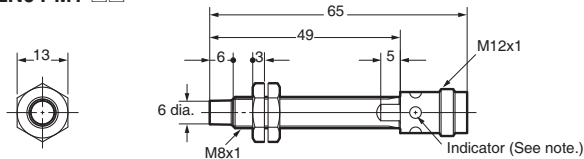
E2A-S08LN04-M1-□□
