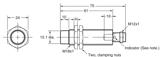
E2A-S18LN16-M1-□
