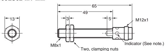
E2A-S08LS02-M1-□□
