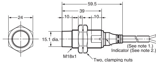
E2A-S18KN16-WP-□
