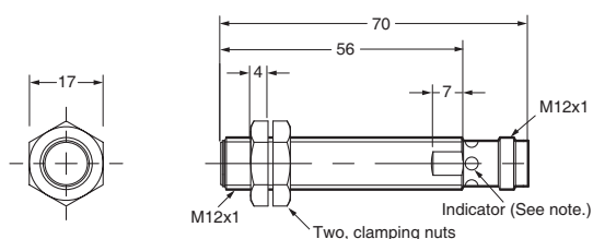
E2A-S12LS04-M1-□
