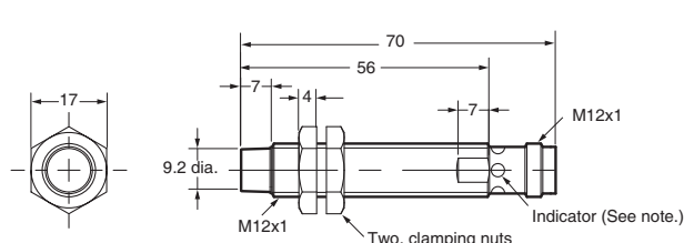
E2A-S12LN08-M1-□
